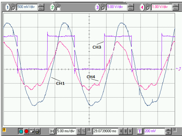
Figure 4. Zero-degree shifted phase references, Phase A Channel: 4. Phase A Line-to-Neutral Voltage 1. Attenuated and Filtered Mains Voltage at RN6-3 3. Reference Comparator Output, TP5
