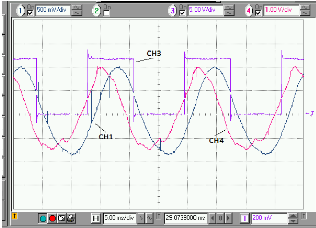
Figure 3. Thirty-degree shifted phase references, Phase A Channel: 4. Phase A Line-to-Neutral Voltage 1. Attenuated and Filtered Mains Voltage at RN6-3 3. Reference Comparator Output, TP5
